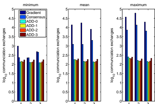
Fig. 4. Min (left), mean (center) and max (right) number of local communications required to reach \|g(\lambda_k)\| \leq 10^{-10} for gradient descent, consensus-based Newton and ADD, computed for 35 trials each on random graphs with 25 nodes and 75 edges(1), 50 nodes and 350 edges(2), and 100 nodes and 1000 edges (3). The min and max are on the same order of magnitude for ADD, demonstrating small variance.
