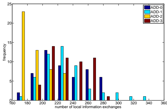
Fig. 3. Histogram of the number of local communications required to reach \|g(\lambda_k)\| \leq 10^{-10} for ADD- N with respect to parameter N , for 50 trials of the network optimization problem on random graphs with 25 nodes and 75 edges. ADD-2 is shown to be the best on average by about 10% indicating that with respect to communication cost, larger N is not necessarily better.
