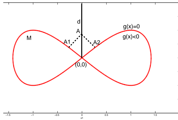
Figure 3: M does not satisfy the LICQ condition and the projection of a point A on the line d has two elements A_1 and A_2 .
