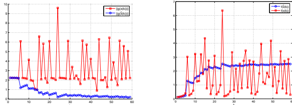
Fig. 3. The figure on the left shows the convergence behavior of the constraint violation for the two primal sequences, \{x_k\} and \{\hat{x}_k\} . Similarly, the figure on the right shows the convergence of the corresponding primal objective function values.
