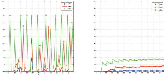
Fig. 2. The convergence behavior of the primal sequence \{x_k\} (on the left) and \{\hat{x}_k\} (on the right).
