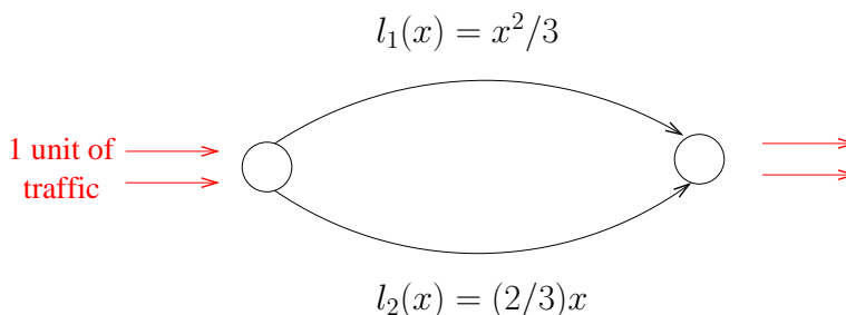
Figure 1: A two link network with congestion-dependant latency functions.
